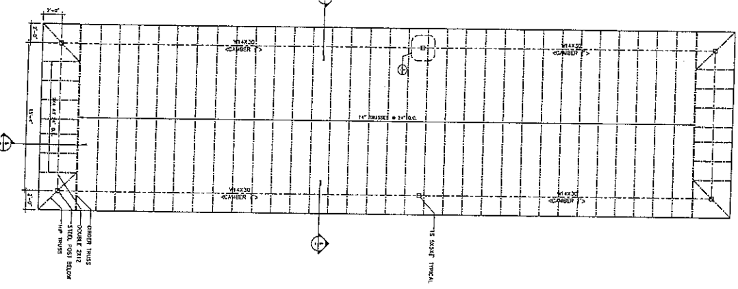
2 CARPORT - ROOF FRAMING 1/4" = 1'-0"
